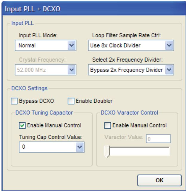
Figure 12. Input PLL + DCXO Window
