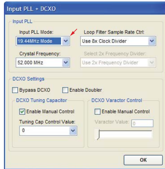
Figure 26. Input PLL + DCXO Window
