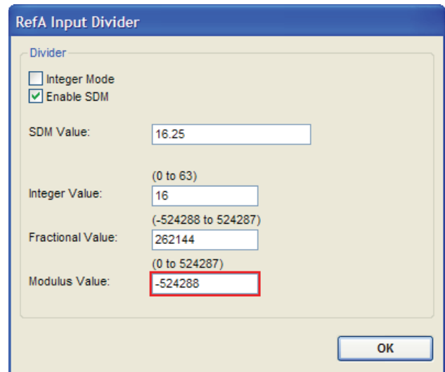
Figure 10. RefA Input Divider Window
