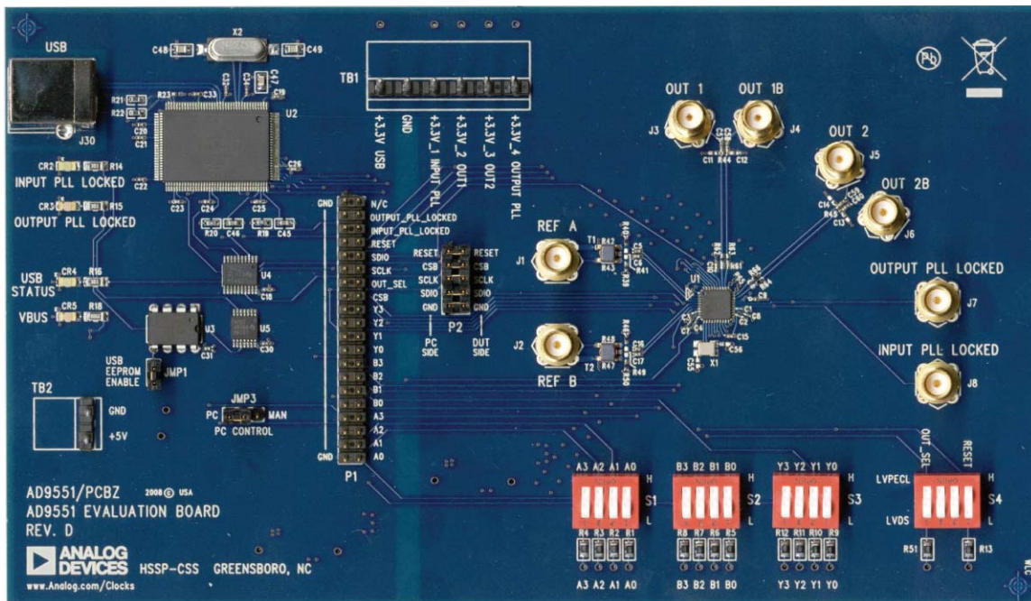
Figure 1. AD9551 Evaluation Board, Revision D
