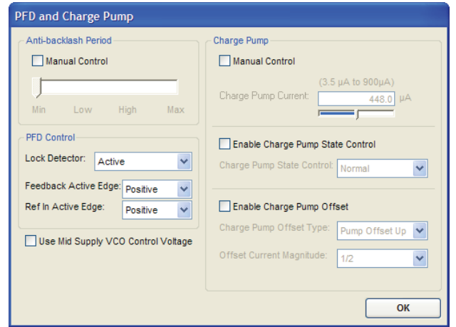
Figure 13. PFD and Charge Pump Window
