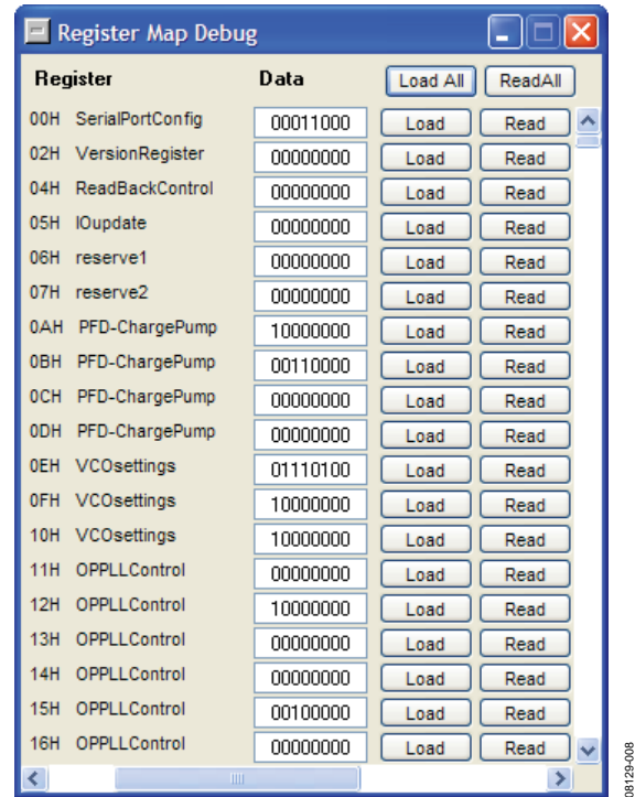
Figure 8. Register Map Debug Window
