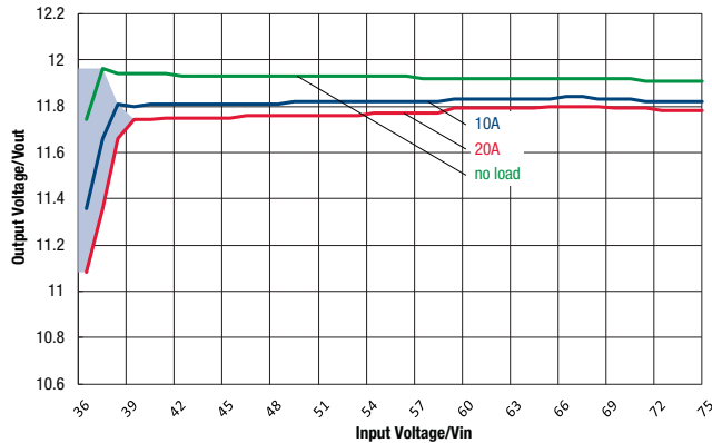
Typical Output Voltage (Vout) vs. Input Voltage (Vin) at +25°C
